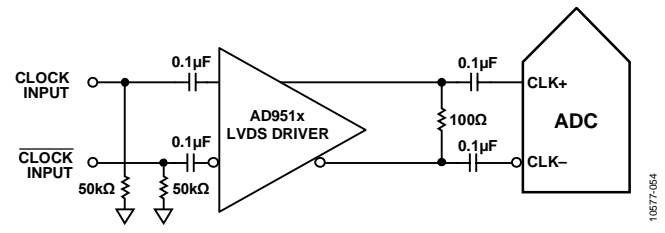
Figure 60. Differential LVDS Sample Clock (Up to 1 GHz)
